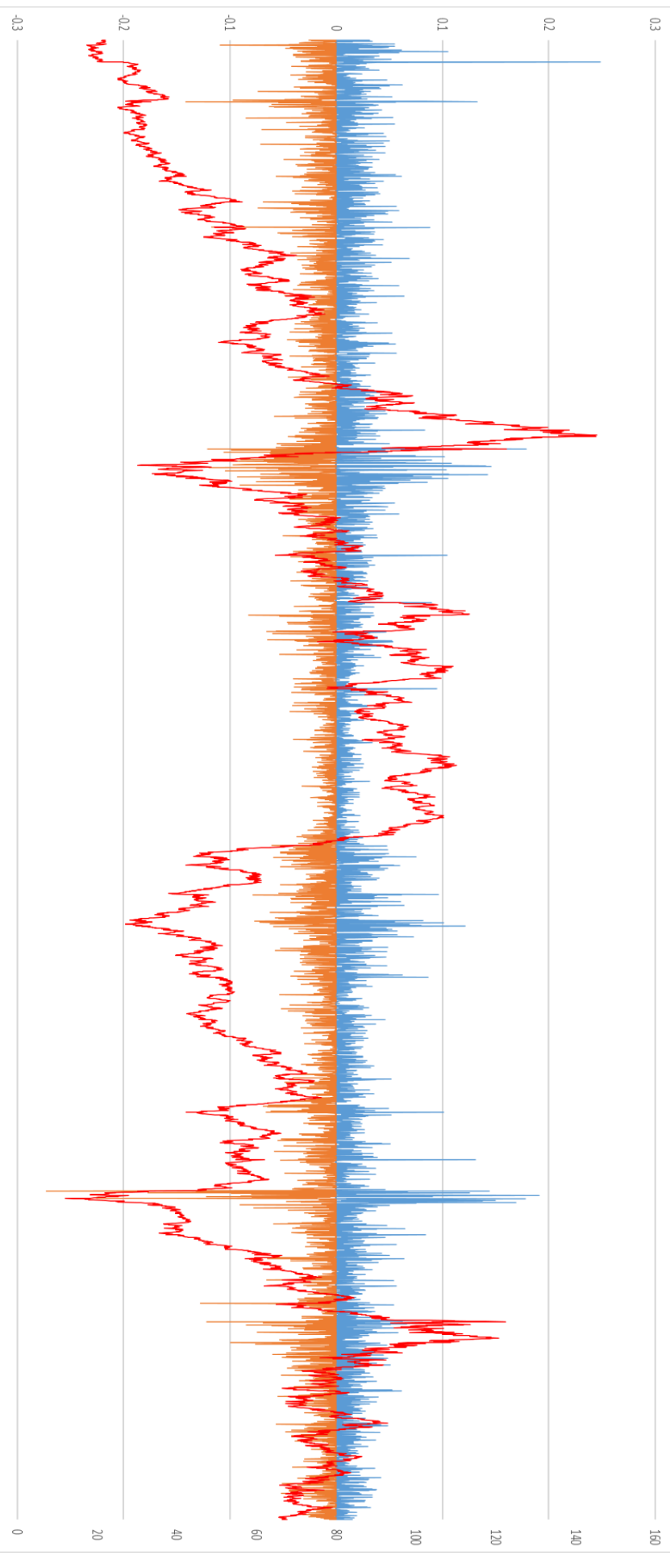
WTIUSD daily
